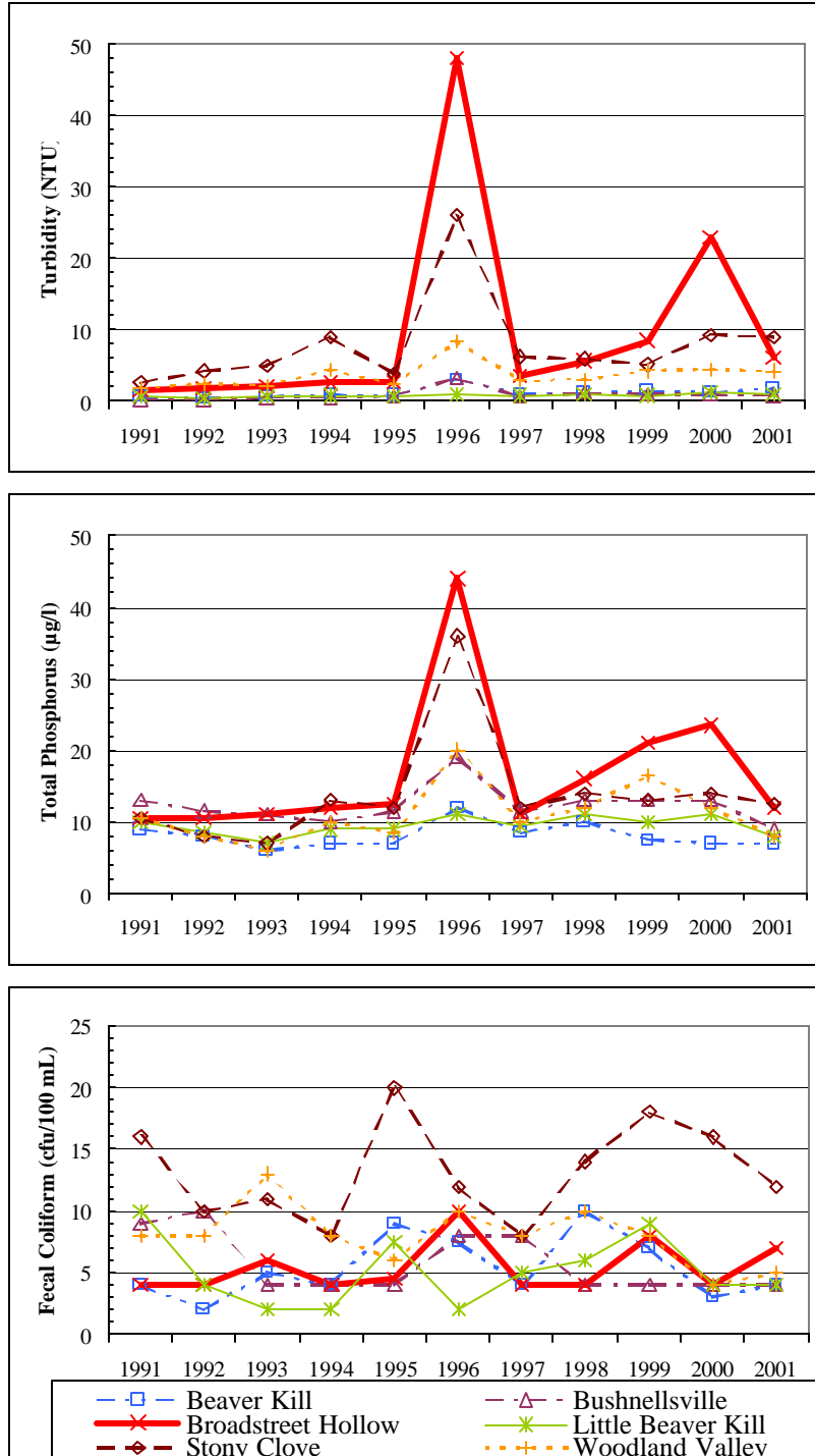
Annual medians for selected water quality analytes for several Catskill streams in the Ashokan basin, 1991-2001.
