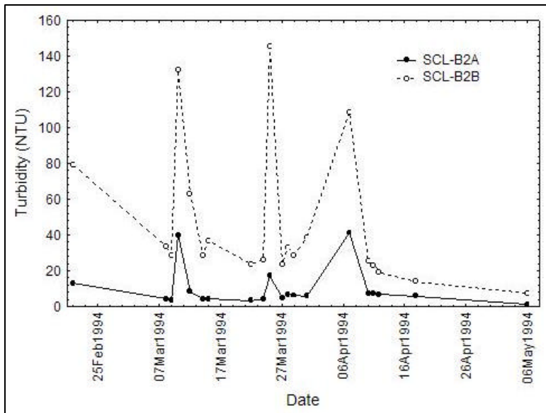
Figure 2 Turbidity readings above and below a large bank failure on the Stony Clove Creek in Chichester, February to May 1994.
